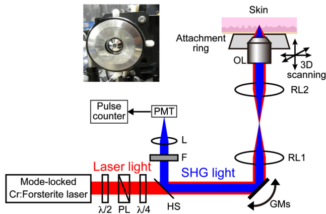
Fig. 2 Experimental setup. \lambda/2 : half-wave plate; PL: polarizer; \lambda/4 : quarter-wave plate; HS: harmonic separator; F: infrared-cut filter; L: lens; PMT: photon-counting-type photomultiplier tube; GMs: galvanometer mirrors; RL1 and RL2: relay lenses; OL: oil-immersion objective lens.
