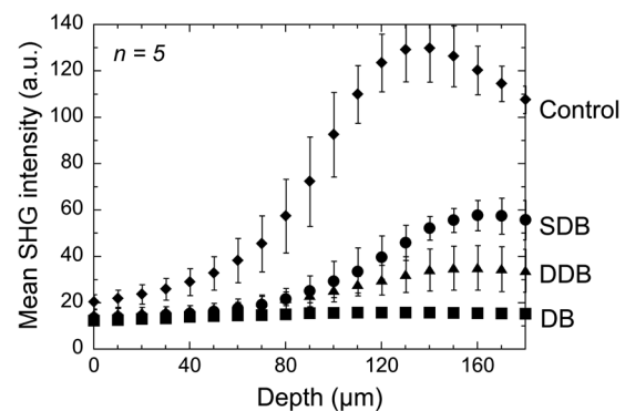
Fig. 6 Dependence of the mean SHG intensity on the probing depth for control, SDB, DDB, and DB samples. Incident laser power was set to 10 mW for each sample.
