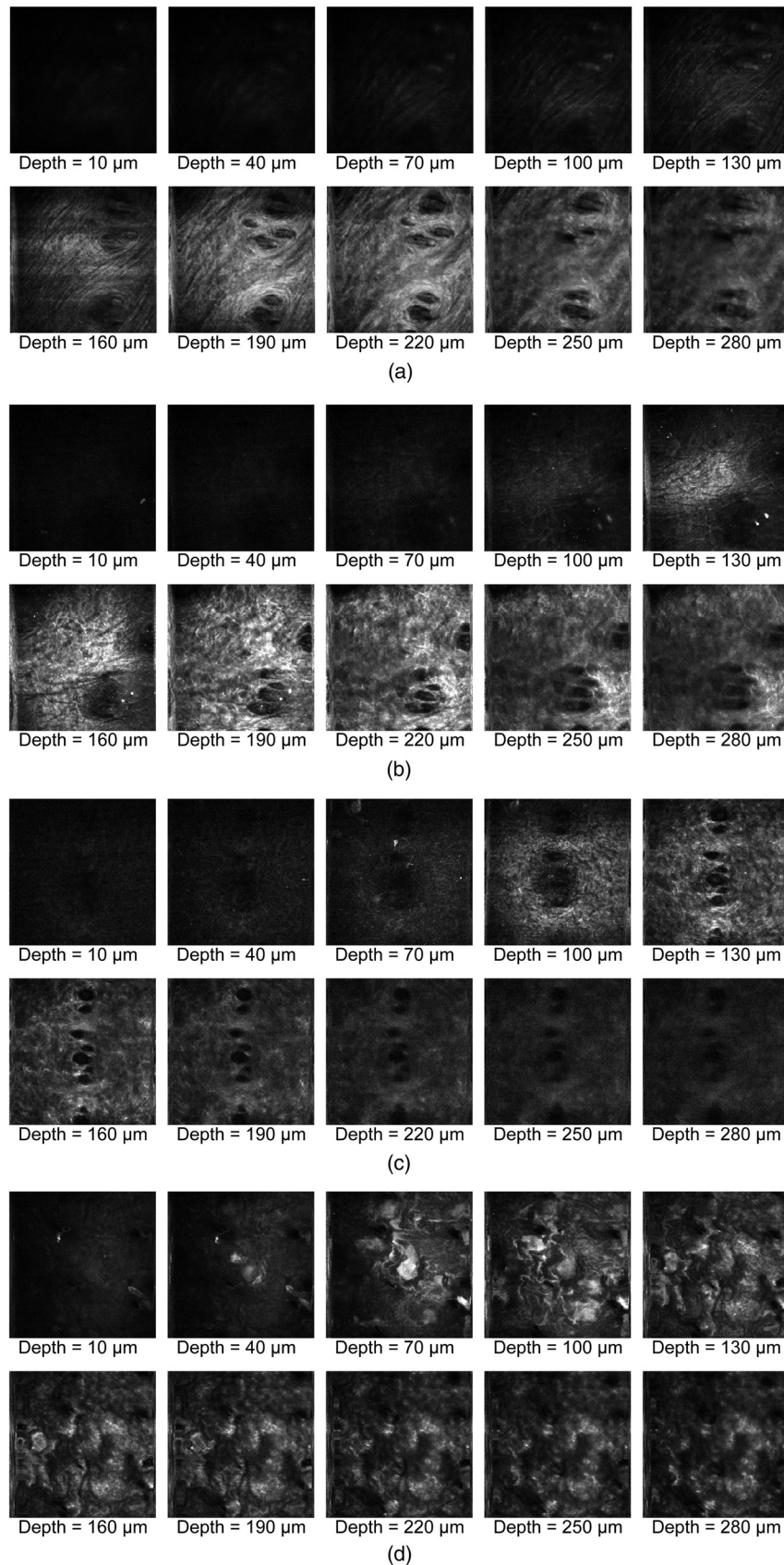
Fig. 3 Depth-resolved SHG images of dermal collagen fiber at a depth from 10 to 280 \mu\text{m} in (a) control, (b) SDB, (c) DDB, and (d) DB samples. Incident laser power was 10 mW for control, 15 mW for SDB, 25 mW for DDB, and 40 mW for DB samples. Image size = 600 \times 600 \mu\text{m}^2 . A series of more precisely depth-resolved SHG images was given in Video 1 (imaged region = 600 \times 600 \mu\text{m}^2 , interval of scanning depth = 10 \mu\text{m} , MOV 1.5 MB) [URL: http://dx.doi.org/10.1117/1.JBO.18.6.061231.1 ].
