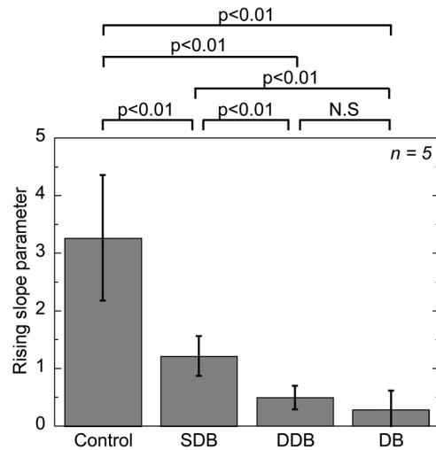
Fig. 7 Comparison of rising slope in SHG depth profile among control, SDB, DDB, and DB samples.
