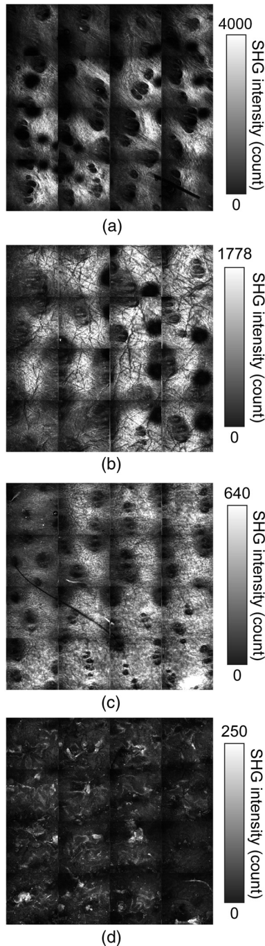
Fig. 4 Large-area SHG images of dermal collagen fiber at a depth of 180\ \mu\text{m} from the skin surface for (a) control, (b) SDB, (c) DDB, and (d) DB samples. SHG intensity is represented by the common gray-scale for all SHG images by considering differences of the incident laser power among samples. Image size = 2.4 \times 2.4\ \text{mm}^2 .
